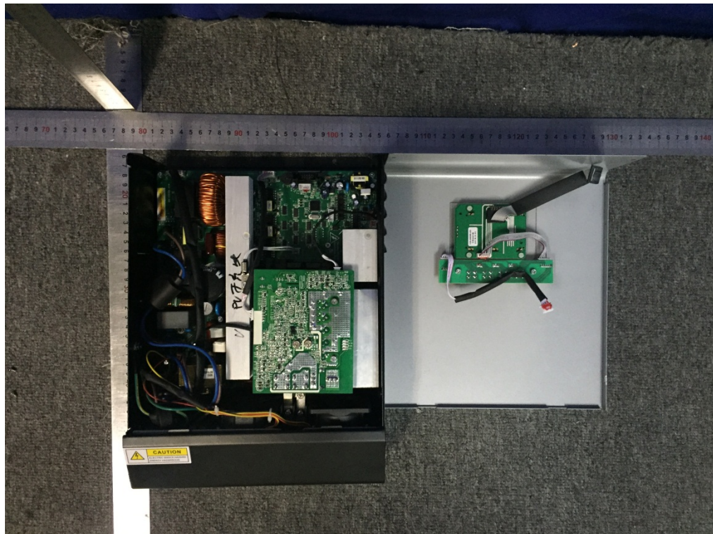
Fig. 5 -- Inside view I
