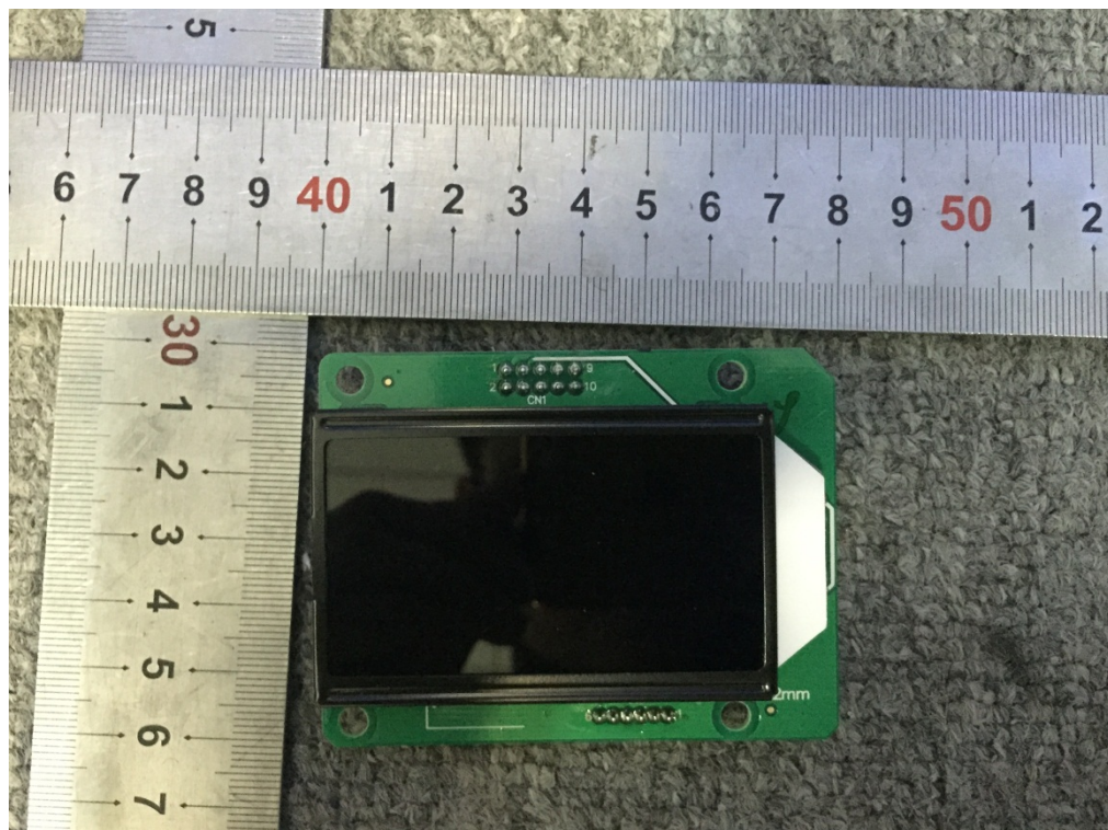
Fig. 16 -- Display board components view
