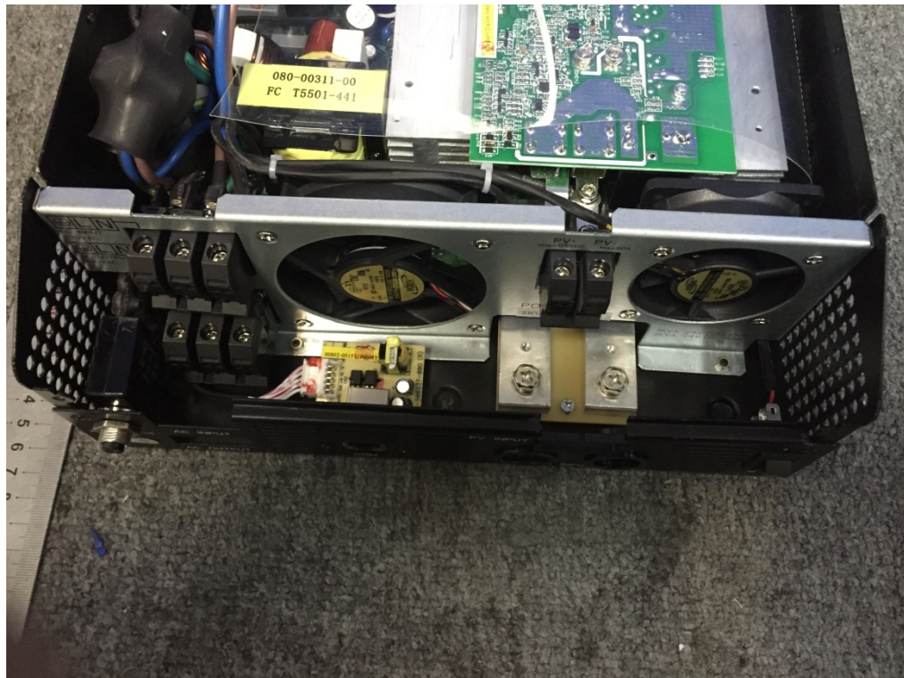
Fig. 7 -- Inside view II
