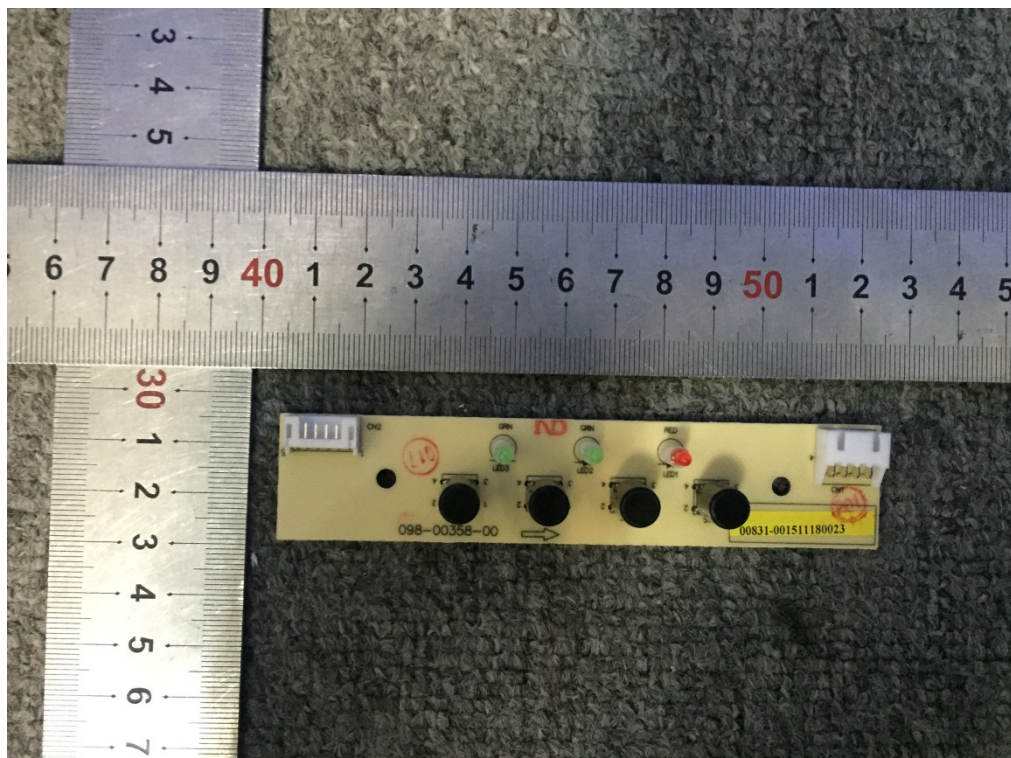
Fig. 14 --Lamp panel board components view
