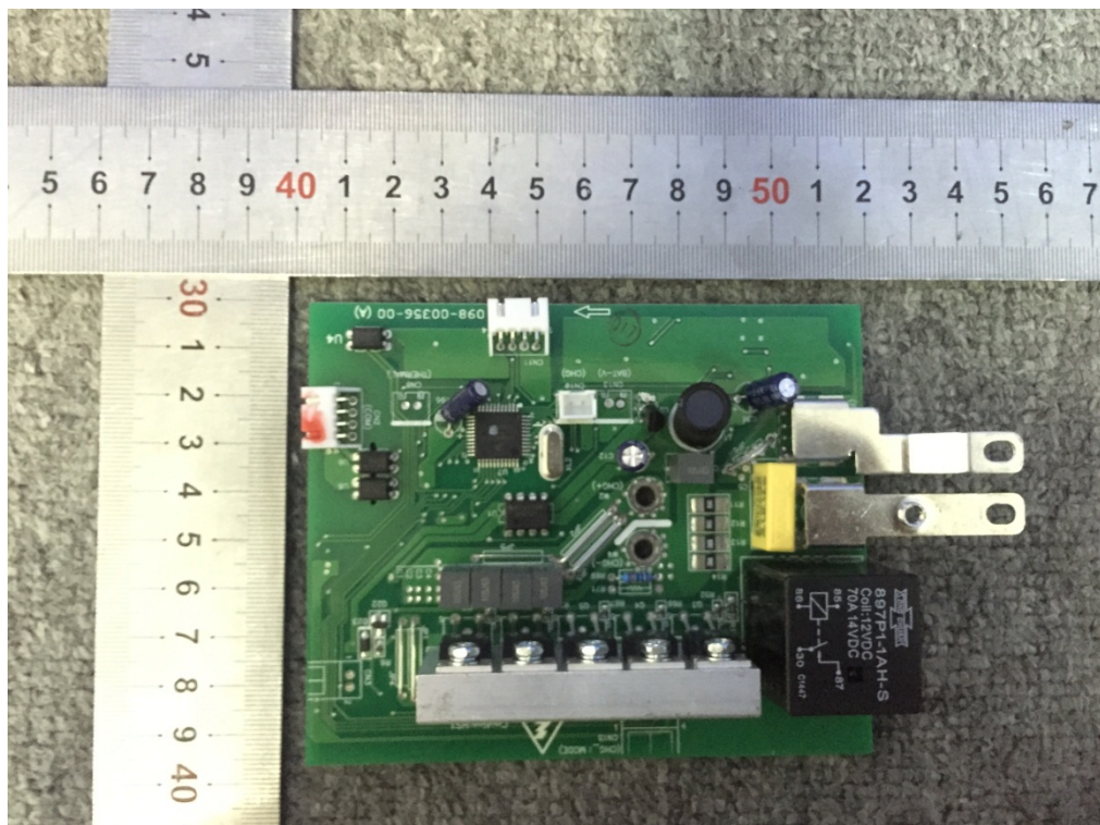
Fig. 8 -- Control board components view
