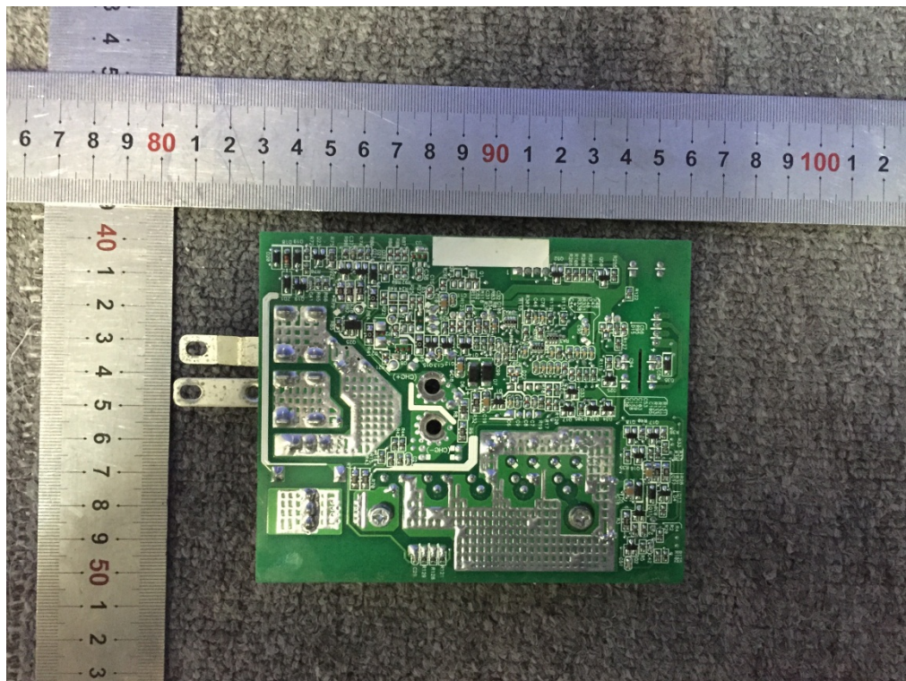
Fig. 9 -- Control board trace view
