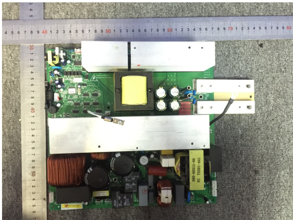
Fig. 10 -- Main Power board components view
