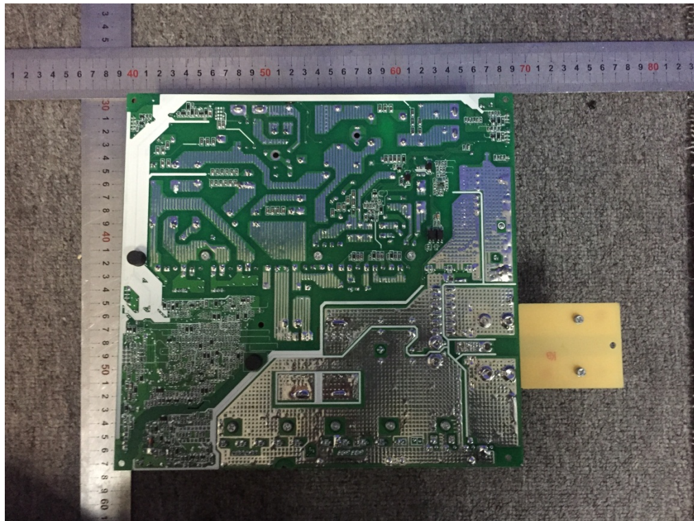
Fig. 11 -- Main Power board components view
