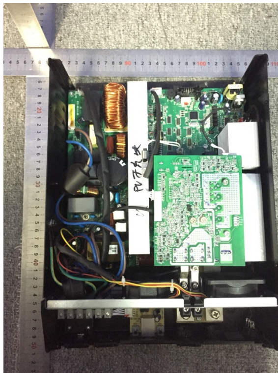
Fig. 6 -- Inside view I
